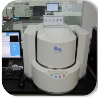
Fluorescence spectrometry
